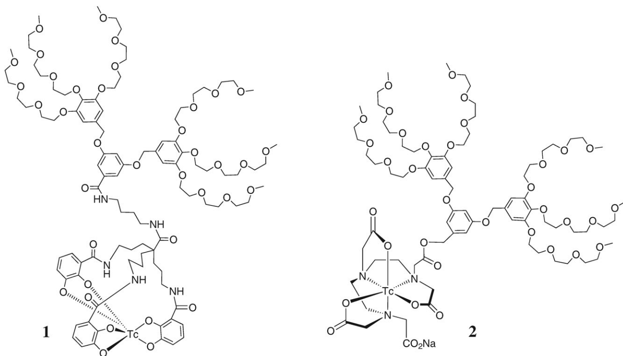
Fig. 1 Proposed structures for dendritic ^{99\text{m}}\text{Tc} chelates 1 and 2 at pH 7.4.
