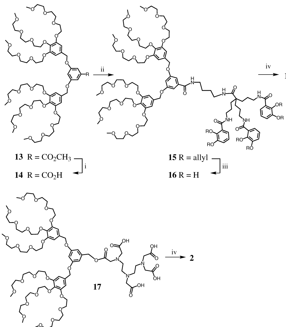
Scheme 2 Synthetic pathways to dendritic complexes 1 and 2 . Reagents and conditions: (i) NaOH, THF–water; (ii) 12 , DCC, DMAP, HOBT, dry \text{CH}_2\text{Cl}_2 , rt; (iii) \text{Pd}(\text{PPh}_3)_4 , THF, \text{NaBH}_4 , HCl, rt; (iv) ^{99\text{m}}\text{TcO}_4^- , \text{SnCl}_2 , ascorbic acid, \text{H}_2\text{O} , rt.
