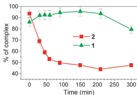
Fig. 2 Stability as a function of time of radiolabelled complexes 1 and 2 measured in buffer PBS (pH 7.4) at 25 °C; error bars of 5%.
