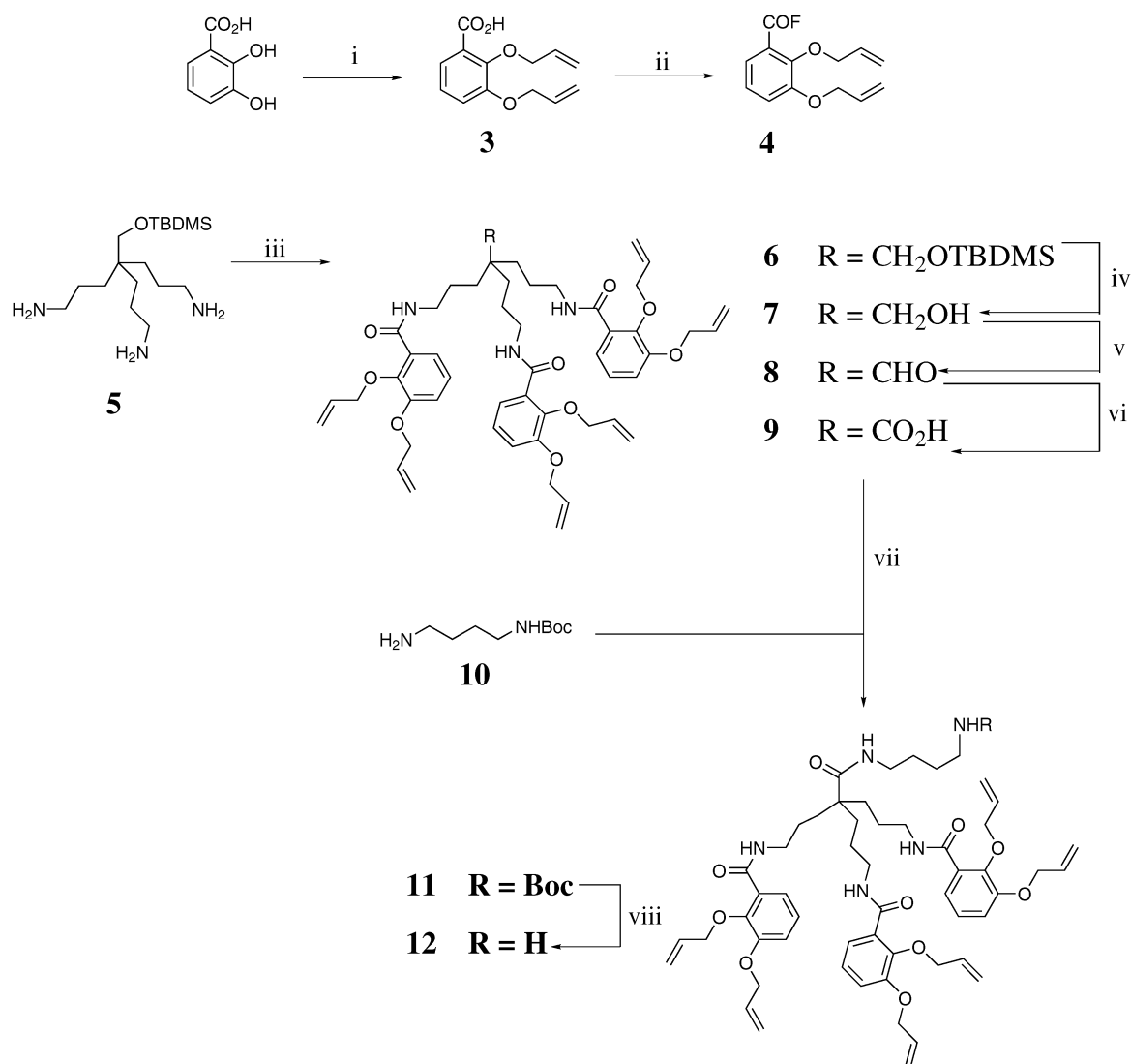
Scheme 1 Synthetic pathway to allyl-protected catecholamide. Reagents and conditions: (i) 1. K 2 CO 3 , allyl bromide, CH 3 CN, reflux then 2. NaOH, EtOH; (ii) trifluorotriazine, pyridine, dry CH 2 Cl 2 , 0 °C, rt; (iii) N,N -diisopropylethylamine, CH 2 Cl 2 , rt; (iv) TBAF, THF, rt; (v) 1. oxalyl chloride, dry DMSO, dry CH 2 Cl 2 , –60 to –40 °C then 2. N,N -diisopropylethylamine, –30 °C to rt; (vi) H 2 NSO 3 H, NaClO 2 , THF–water, rt; (vii) DCC, DMAP, HOBT, CH 2 Cl 2 , rt; (viii) TFA, CH 2 Cl 2 , rt.
